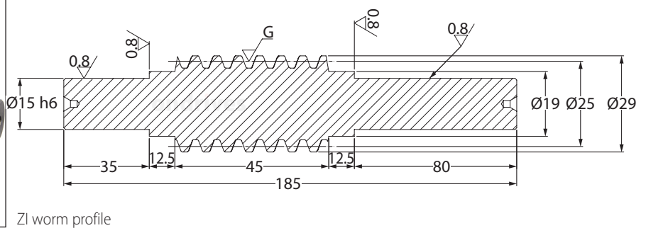
UPSW Shaft Worm
