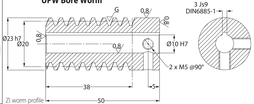
UPW Bore Worm
